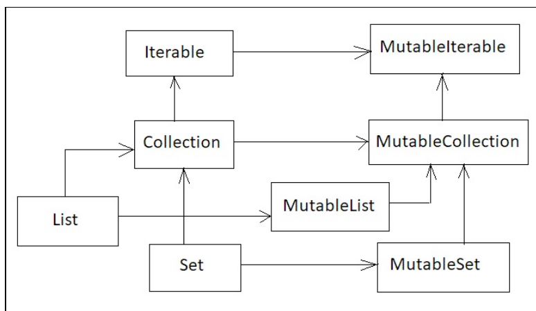
Kotlin collection interfaces hierarchy
