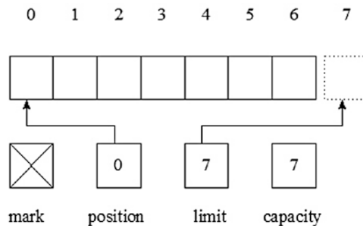
Figure 13-1. The logical layout of a byte-oriented buffer includes an undefined mark, a current position, a limit, and a capacity
